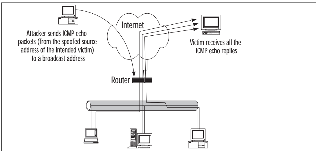
Figure 3.1 Diagram of a smurf attack.
